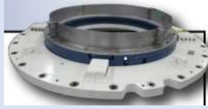
Radial seals Turbine pressure up to 60 PSI (400 kPa)
